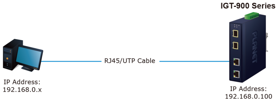
Figure 3-3: Web Management
